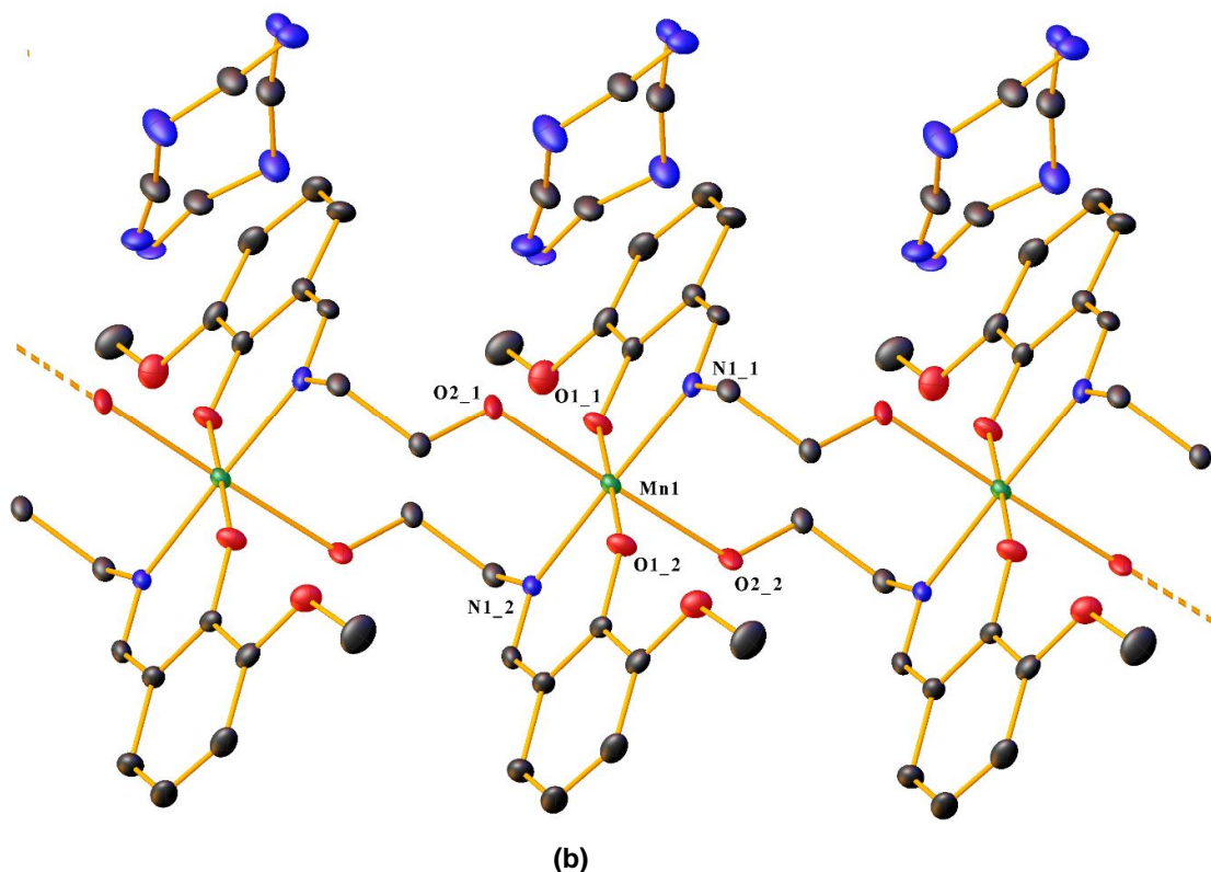
Figure 1. (a) Crystal structure of the Mn(III) complex. Displacement ellipsoids are drawn at the 30% probability level. (b) Drawing of the coordination polymer. H atoms are omitted for clarity.
