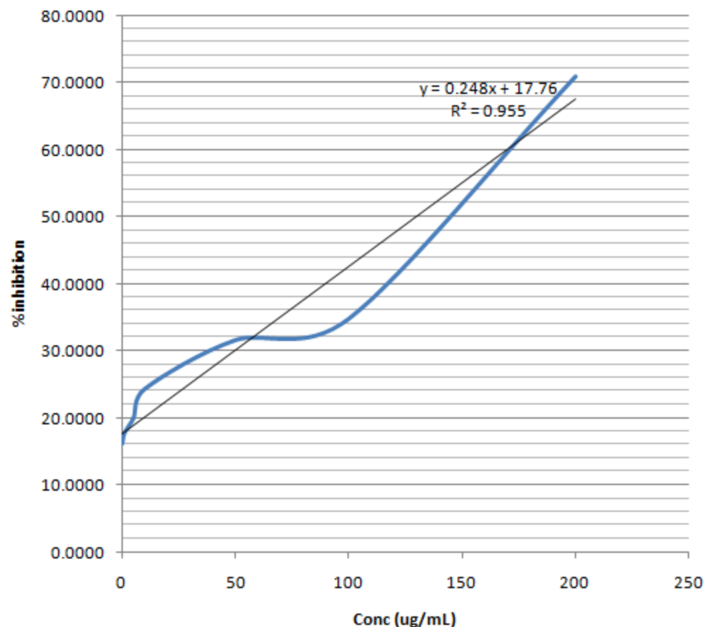
Figure 1: Percentage Inhibition against Concentration (0-200 \mu\text{g/mL} ) of Standard Ascorbic Acid
