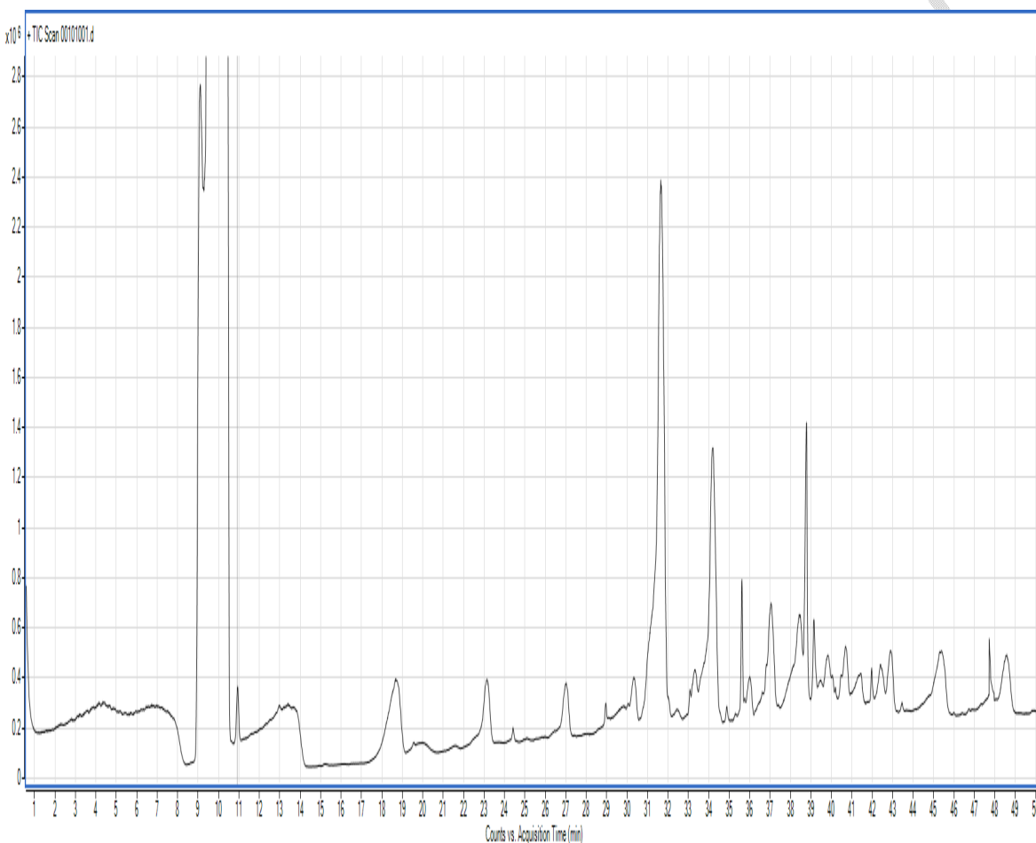
Fig 3: GC-MS Chromatogram of EtOAc Fraction of A. sieberiana
