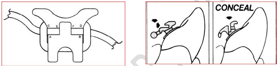
Fig. 3.a Conceal brackets have three different arch wire slot widths for the three different . insertion B: Occlusal insertion. tip A-B, torque E-F, and rotation C-F or E-D
