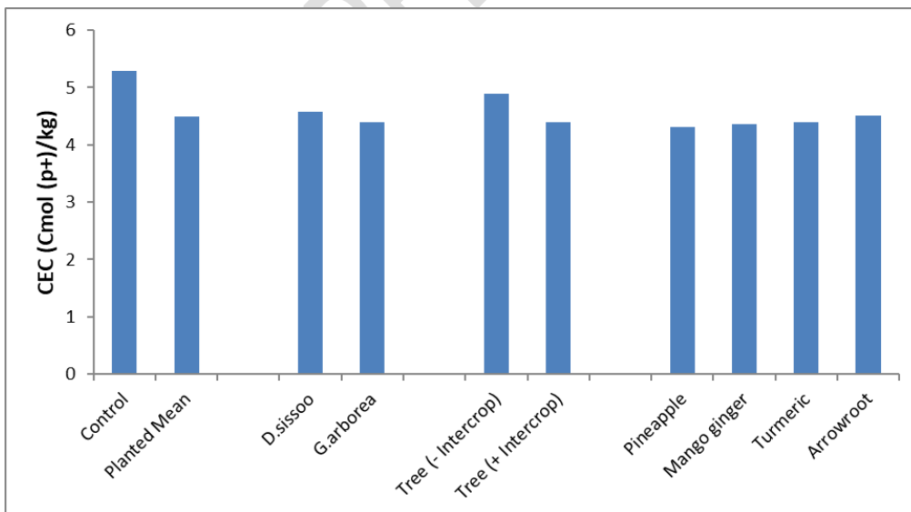
Fig.6. Contrasting of CEC at surface soil (0-15cm)
