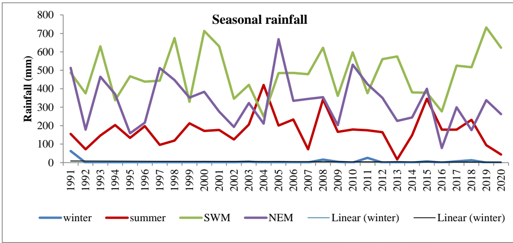
Figure 2. Trend in seasonal rainfall over 30 years
