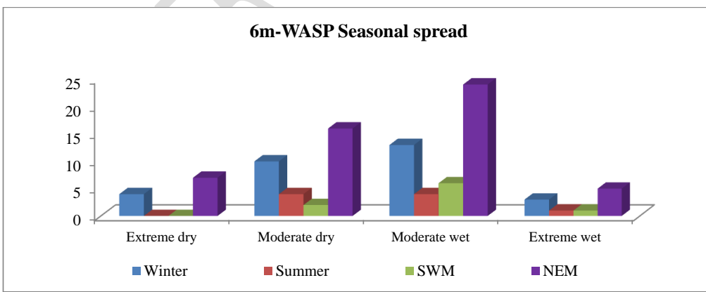
Figure 7. Occurrence dry and wet events over different seasons with 6m-WASP
