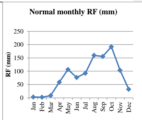
Figure 3: Monthly rainfall normal (30 years average) over the study region
