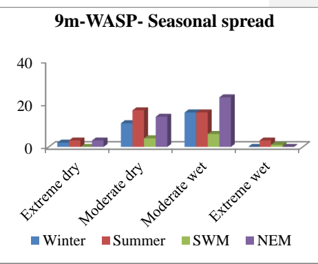
Figure 9. Occurrence dry and wet events over different seasons with 9m-WASP
