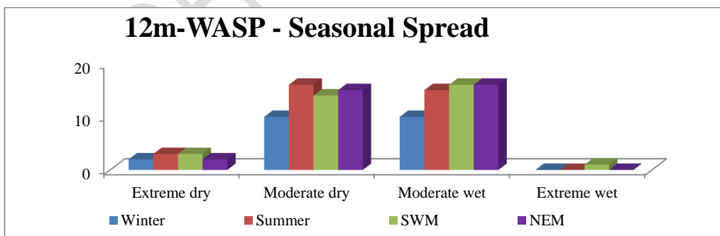
Figure 11. Occurrence dry and wet events over different seasons with 12m-WASP
