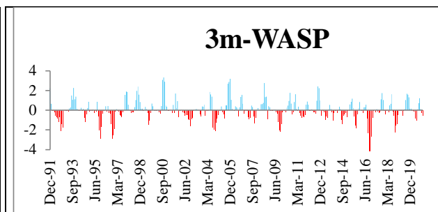
Figure 4. The wet and dry spells over 30years periods with 3m-WASP.
