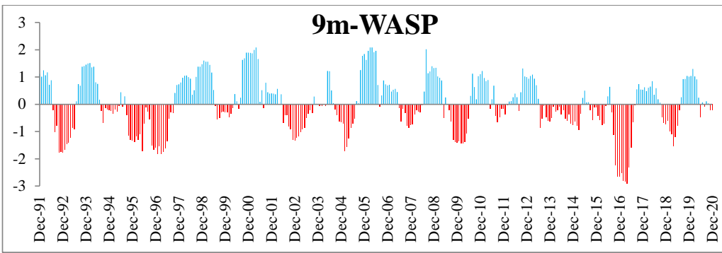
Figure 8. The wet and dry spells over 30years periods with 9 m-WASP
