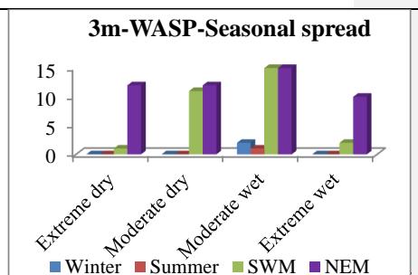
Figure 5. Occurrence dry and wet events over different seasons with 3m-WASP
