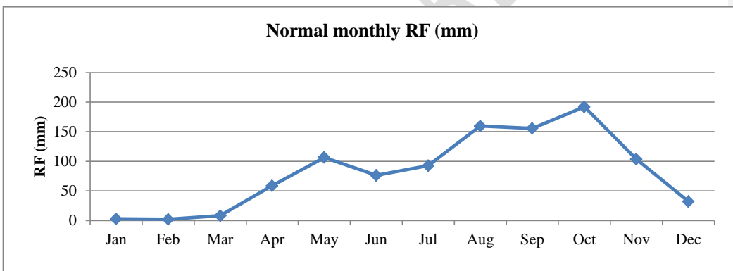
Figure 3. Monthly rainfall normal (30 years average) over the study region
