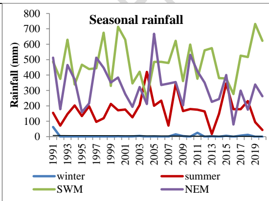
Figure 2: Trend in seasonal rainfall over 30 years
