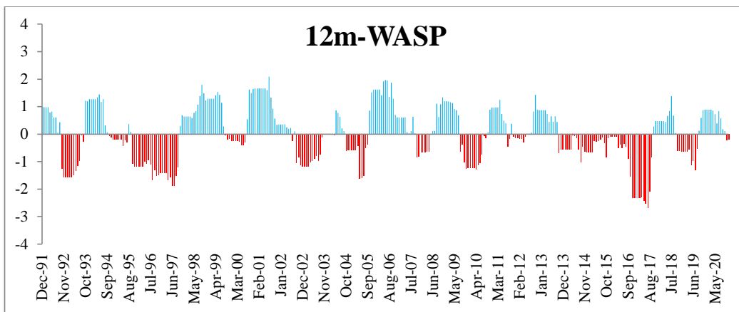
Figure 10. The wet and dry spells over 30years periods with 12m-WASP
