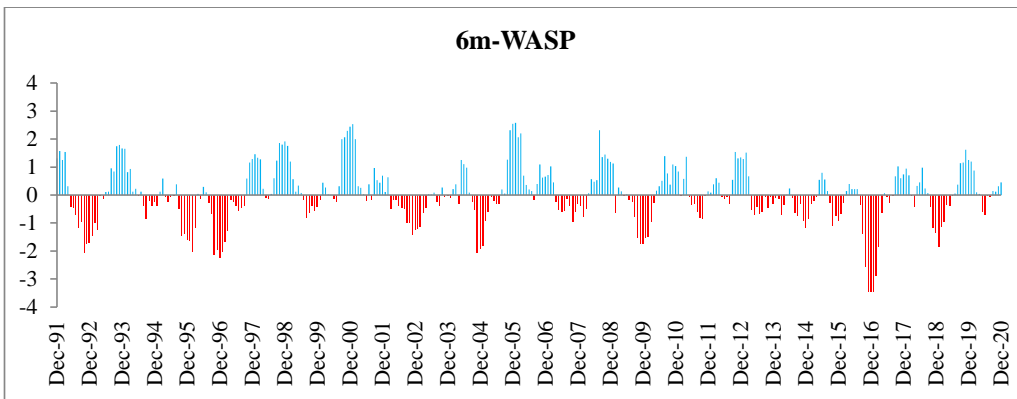
Figure 6. The wet and dry spells over 30years periods with 6m-WASP
