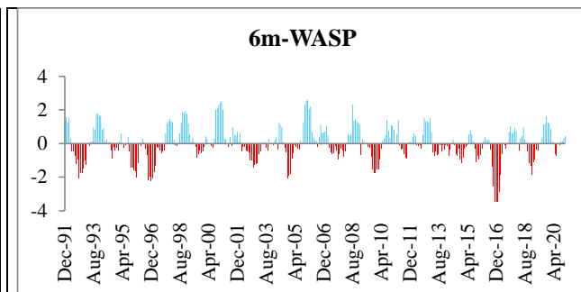
Figure 6. The wet and dry spells over 30years periods with 6m-WASP.
