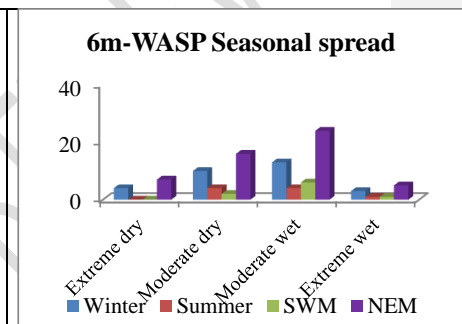
Figure 7. Occurrence dry and wet events over different seasons with 6m-WASP
