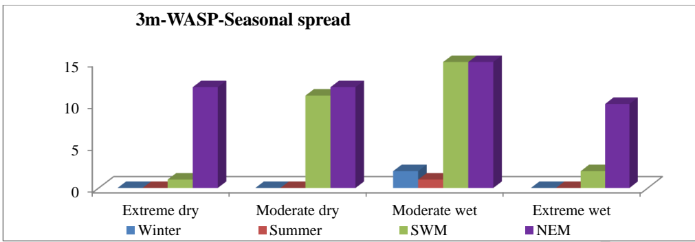
Figure 5. Occurrence dry and wet events over different seasons with 3m-WASP
