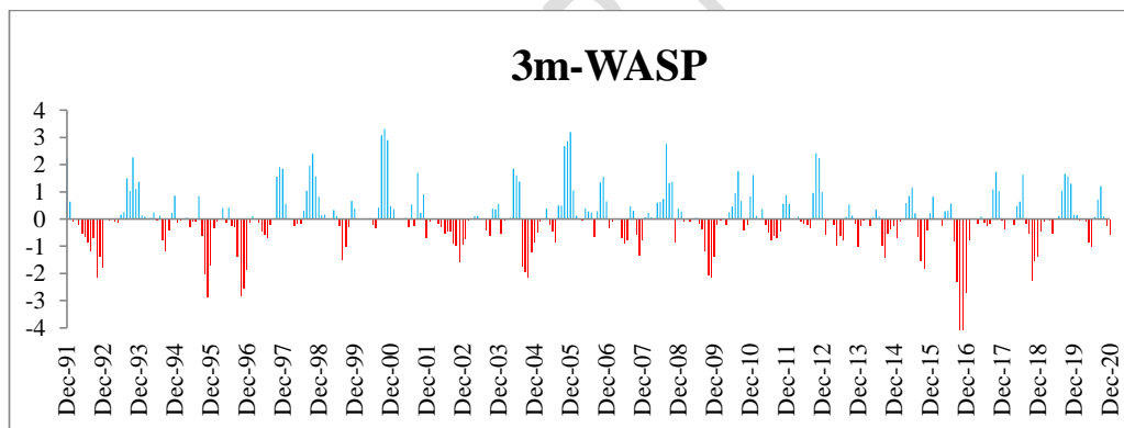
Figure 4. The wet and dry spells over 30years periods with 3m-WASP.
