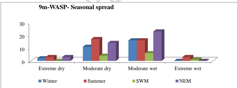
Figure 9. Occurrence dry and wet events over different seasons with 9m-WASP
