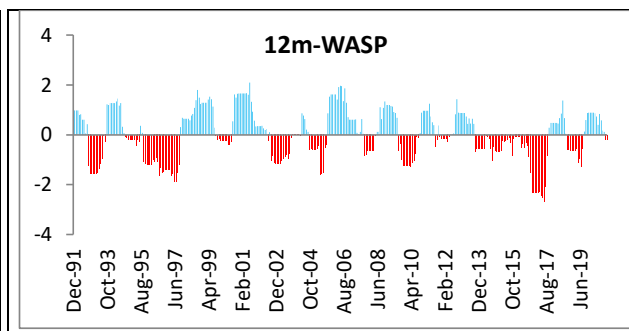
Figure 10. The wet and dry spells over 30 years periods with 12m-WASP
