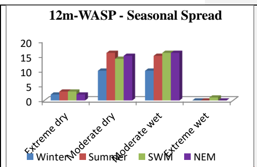
Figure 11. Occurrence dry and wet events over different seasons with 12m-WASP
