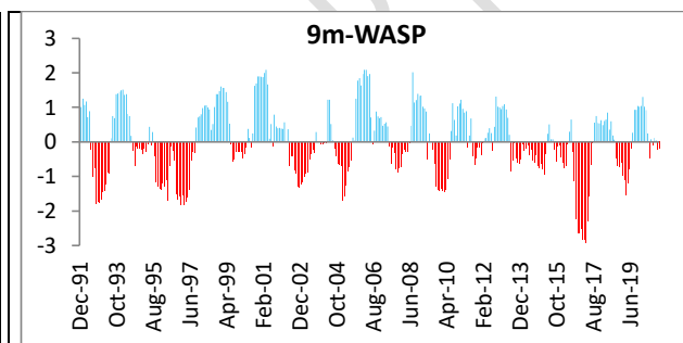
Figure 8. The wet and dry spells over 30years periods with 9 m-WASP
