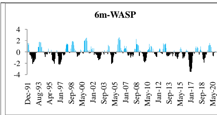
Figure 6. The wet and dry spells over 30years periods with 6m-WASP.
