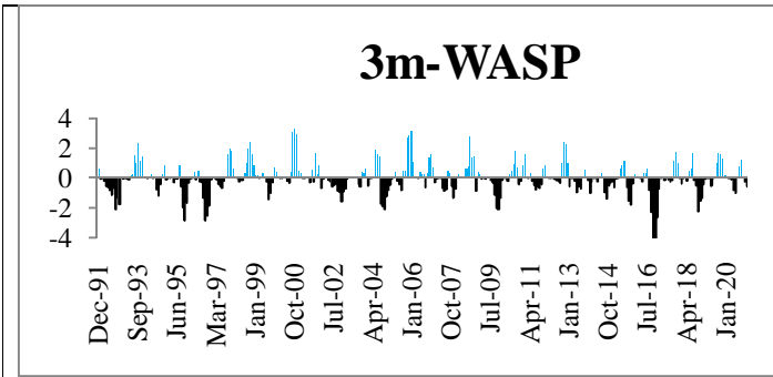
Figure 4. The wet and dry spells over 30years periods with 3m-WASP.
