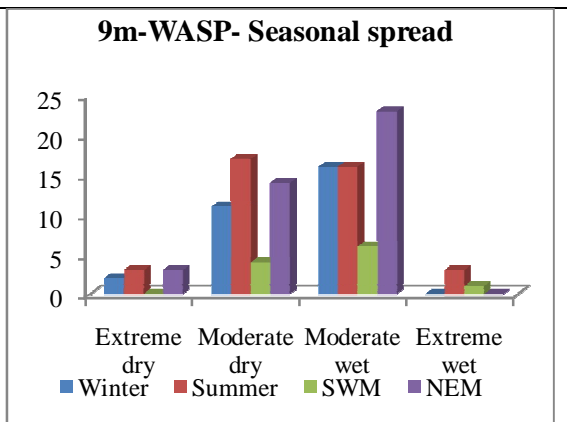
Figure 9. Occurrence dry and wet events over different seasons with 9m-WASP
