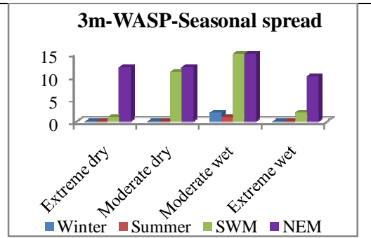
Figure 5. Occurrence dry and wet events over different seasons with 3m-WASP
