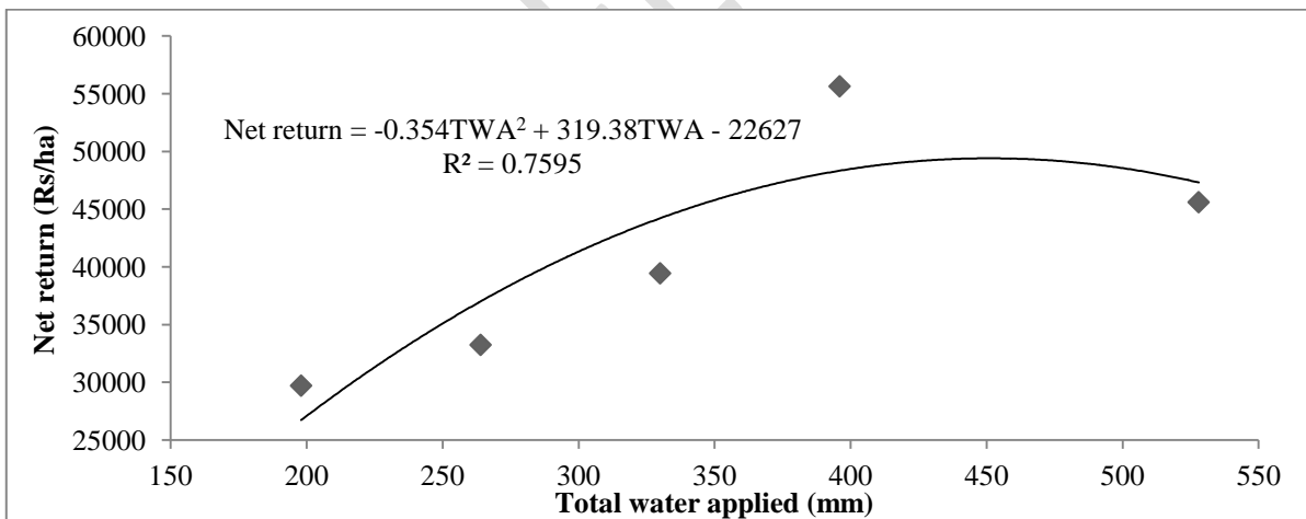
Fig. 6. Relationship between total water applied and net return as influenced by factor of energy balance
