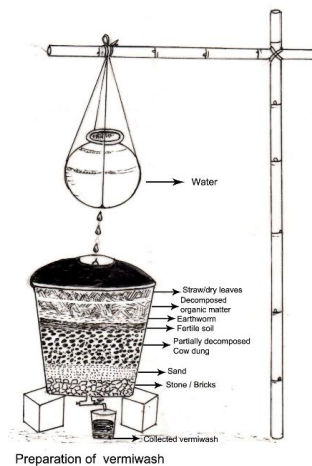
Fig 2: Vermiwash unit (in buckets) for commercial production
