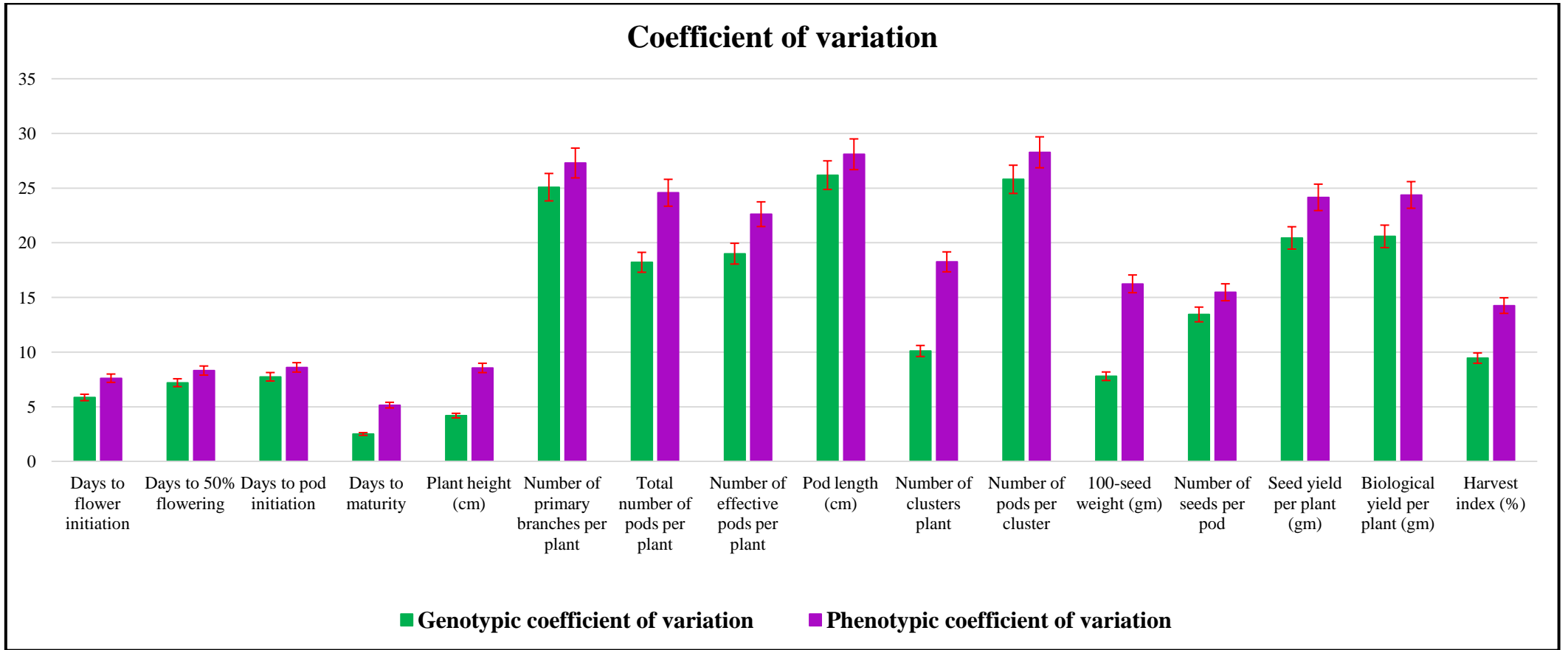
Figure 1: Genotypic coefficient of variation and phenotypic coefficient of variation for different quantitative traits of Greengram
