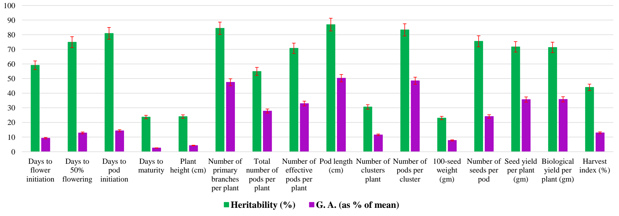
Figure 2: Heritability broad sense (%) and Genetic advance (as % of mean) for different quantitative traits of Greengram
