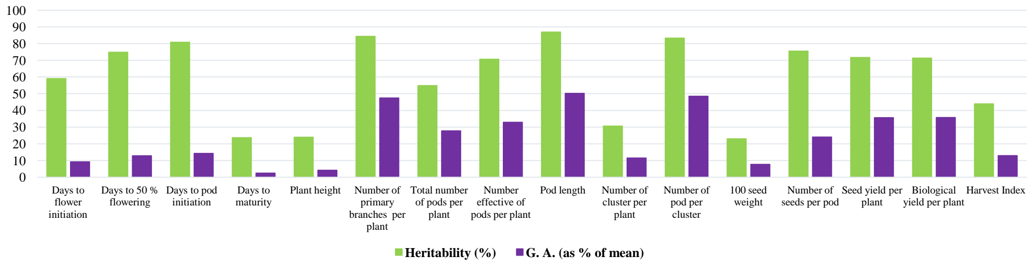
Figure 2: Heritability broad sense (%) and Genetic advance (as % of mean) for different quantitative traits of Greengram
