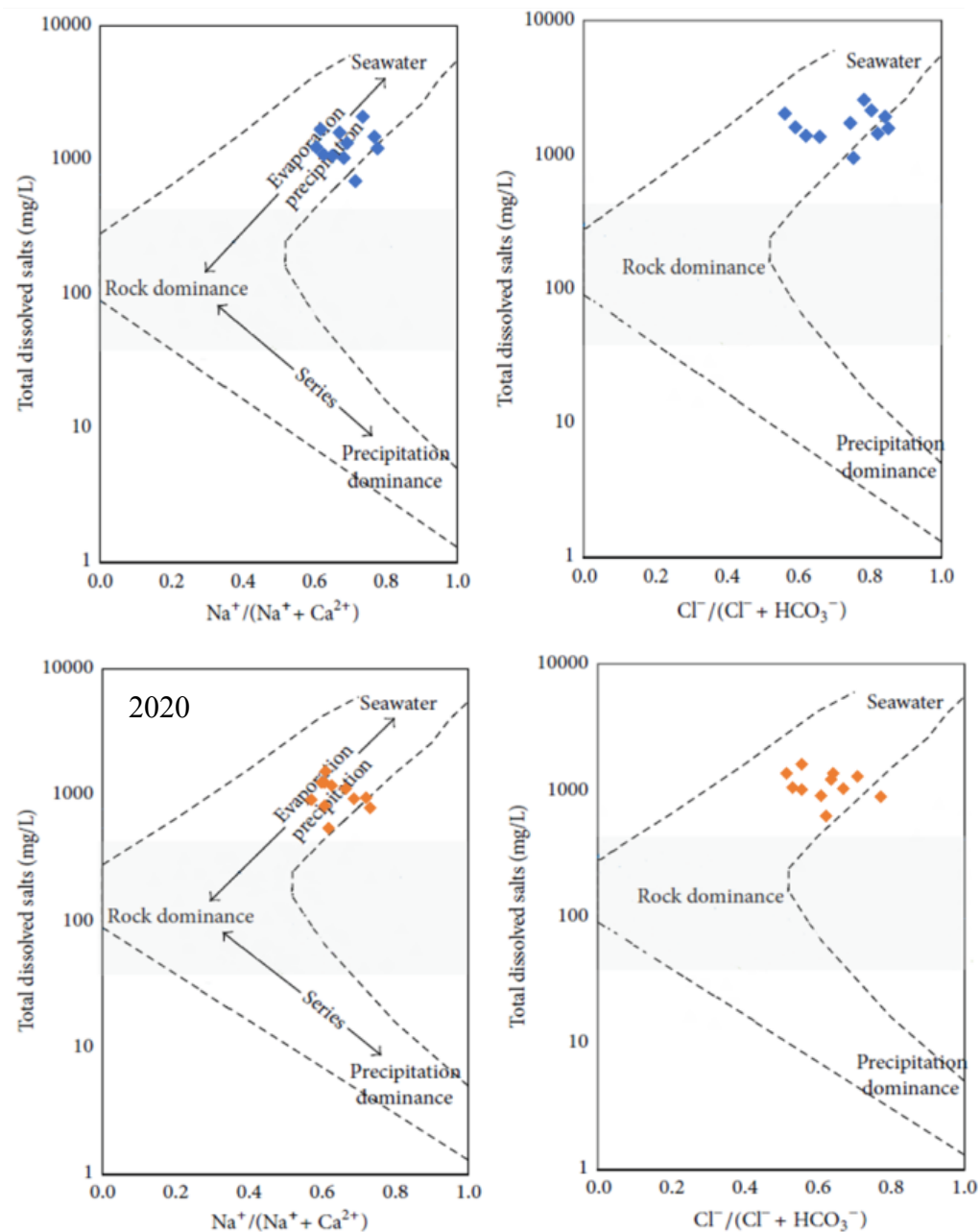
Fig. 4 Gibbs diagram in 2005 and 2020
