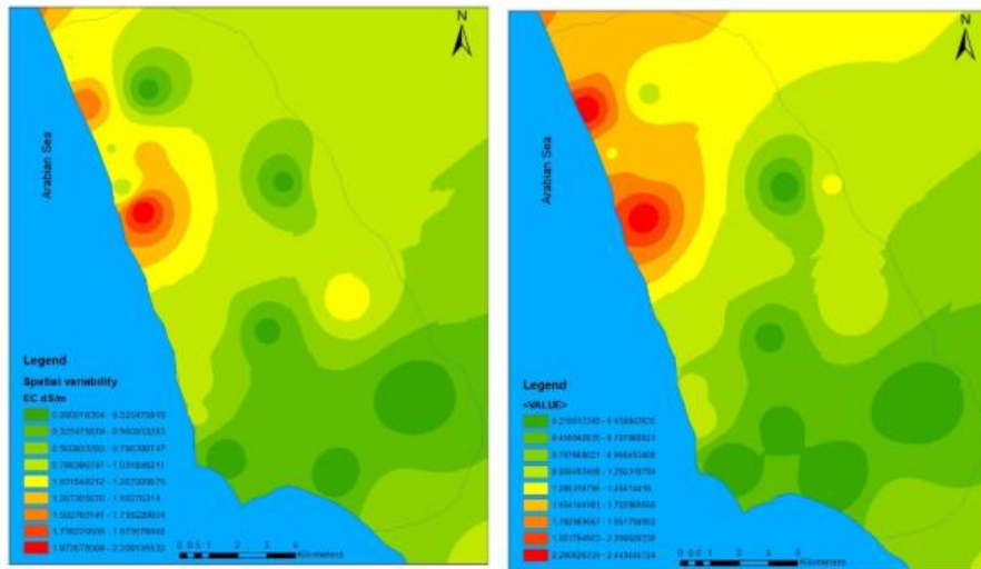
Fig. 8 Spatial variability map of the EC in the confined aquifer
