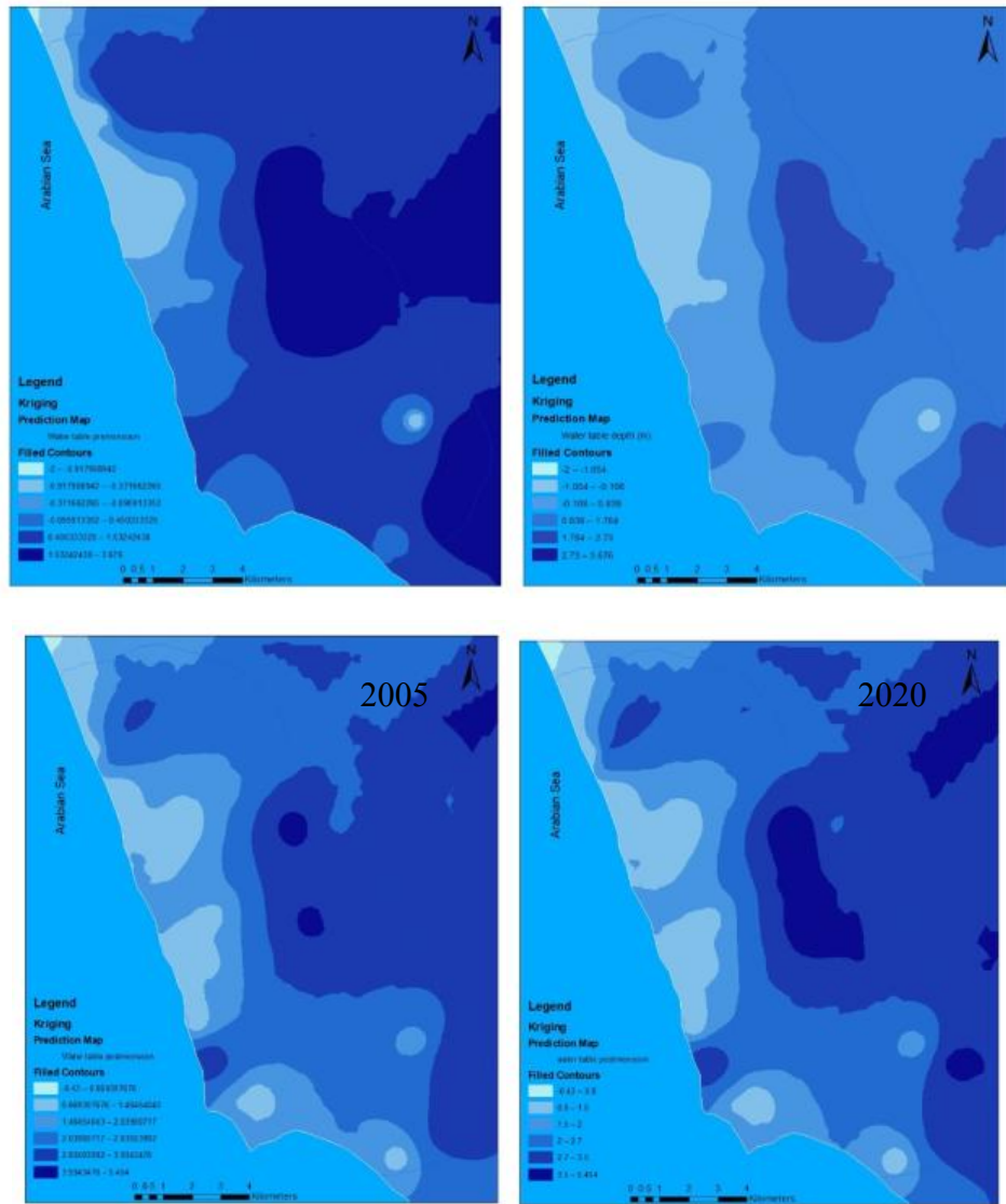
Fig. 7 Spatial variability map of the water table in the semi-confined aquifer
