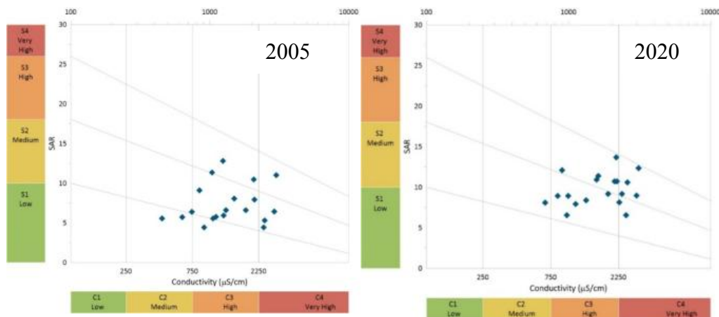
Fig. 5 USSSL diagram in 2005 and 2020
