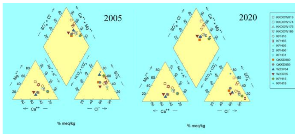
Fig. 3 Hydrochemical facies in 2005 and 2020
