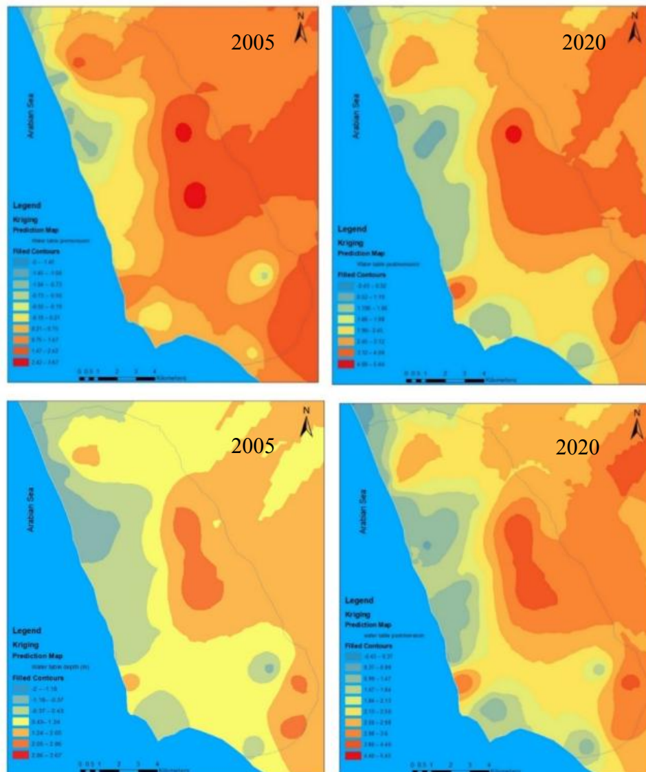
Fig. 6. Spatial variability map of the water table in the confined aquifer
