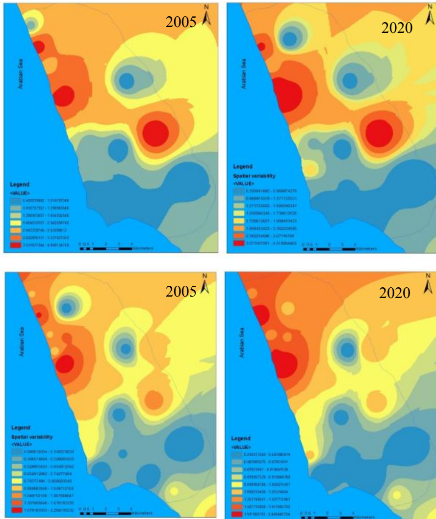
Fig. 9 Spatial variability map of the EC in the semi-confined aquifer
