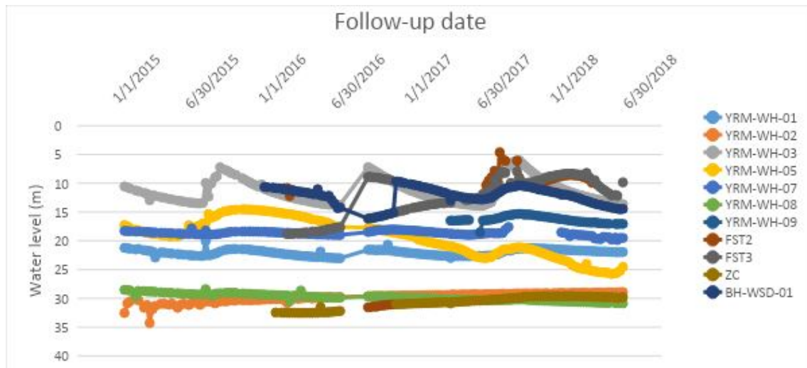
Figure 7: Fluctuation of piezometric levels in the structures of the study area
