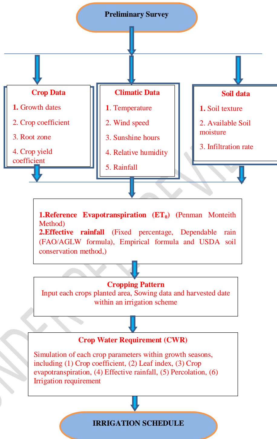
Fig. 2 Flowchart for estimation of crop water requirement in CROPWAT 8.0 (Bhat, et al., 2017)
