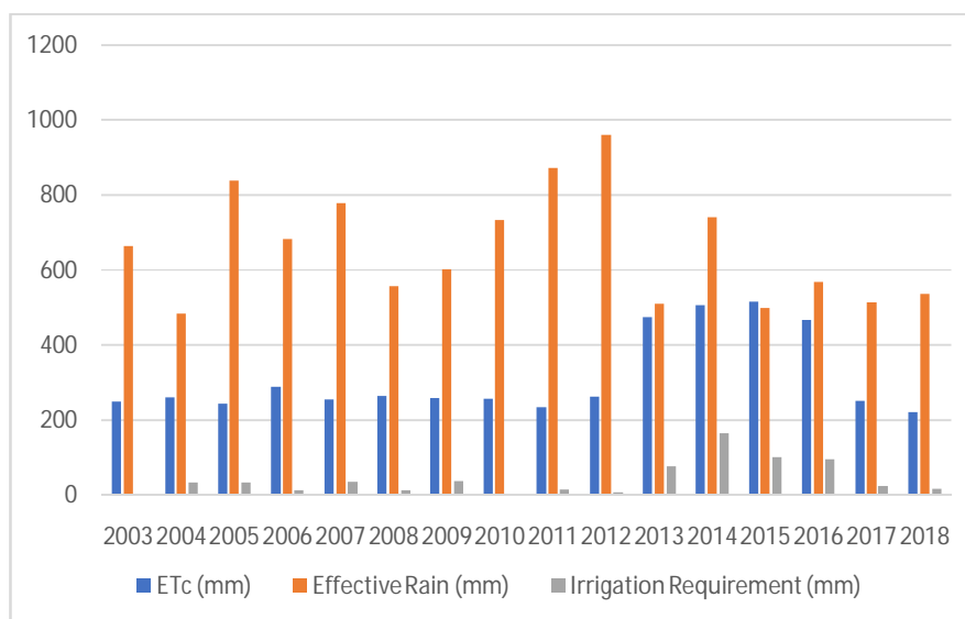
Fig.8. Crop evapotranspiration, Effective rain, and Irrigation Requirements for Kharif Maize in Bilaspur district
