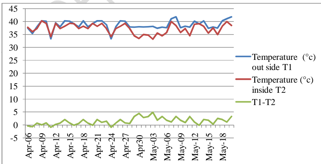
Fig 5. Variation of temperature inside and outside of polyhouse at 04:30 Pm
