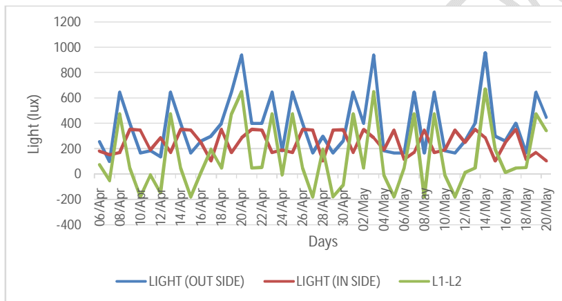
Fig 9. Variation of Light inside and outside of polyhouse at 08:30 Am
