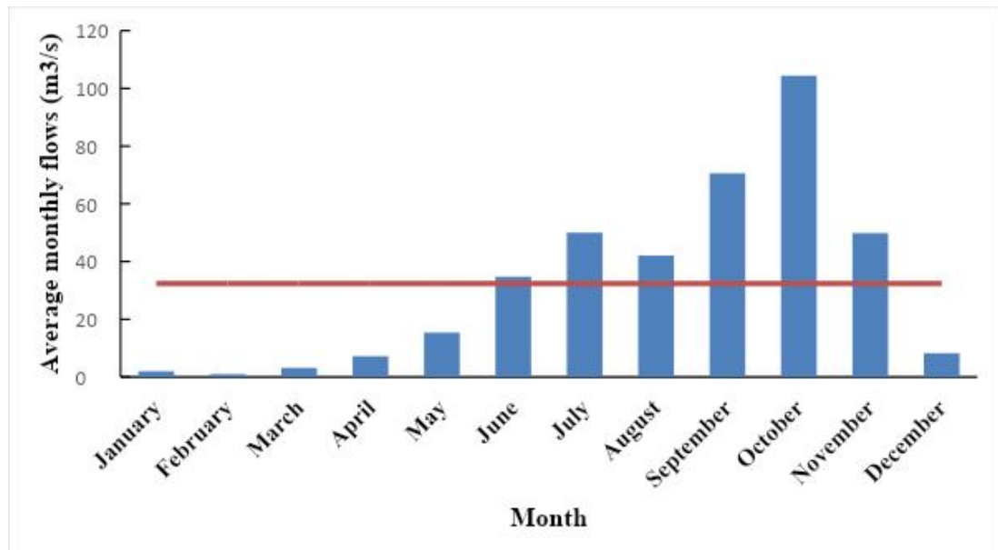
Figure 3. Analysis of the hydrological regime of the N'zi (Bandama) at Dimbokro (1991-2020)
