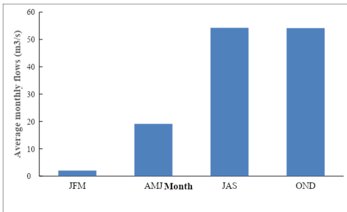
Figure 4. Quarterly mean flows of the N'zi (Bandama) at Dimbokro (1991-2020)
