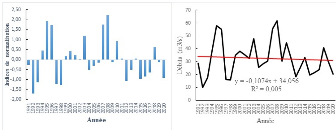
Figure 2. Trends in mean annual flows (m3/s) of the N'zi (Bandama) at Dimbokro (1991-2020)
