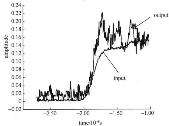
Fig.4 Experimental results by using E5071C Network Analyser.
