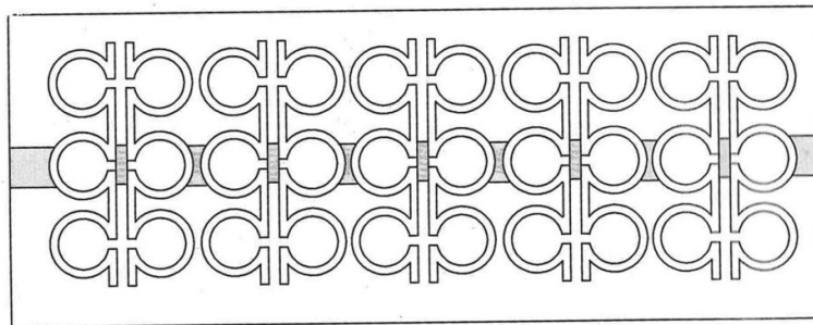
Fig 3. The structure chart of the microstrip transmission line with complementary omega-like structures etched in the ground plane. The gray strip is the microstrip transmission line at the reverse side of printed circuit board.
