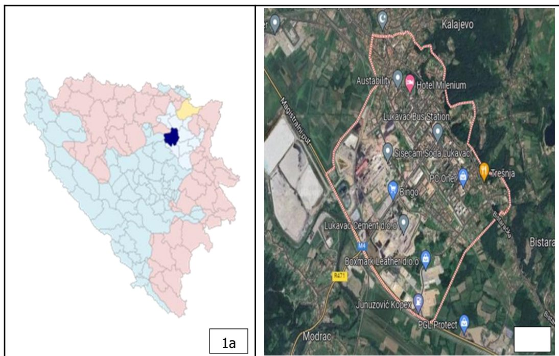
Figure 1. Geographical location of the researched area 1a) the geographical position of the municipality of Lukavac in Bosnia and Herzegovina 1 b) research area (source: Google maps application)
