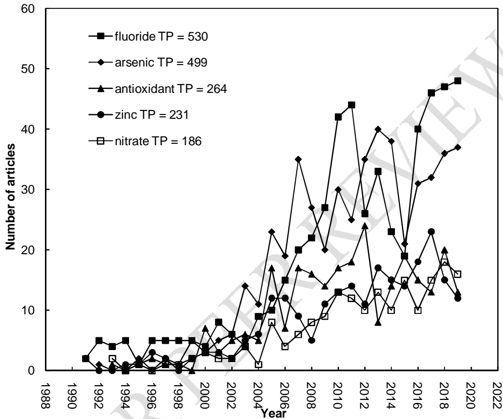
Figure 6. Development trends of the five main pollutants
