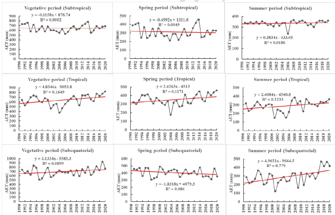
Figure 4: Evolution of real evapotranspiration (AET) over the period 1991-2020
