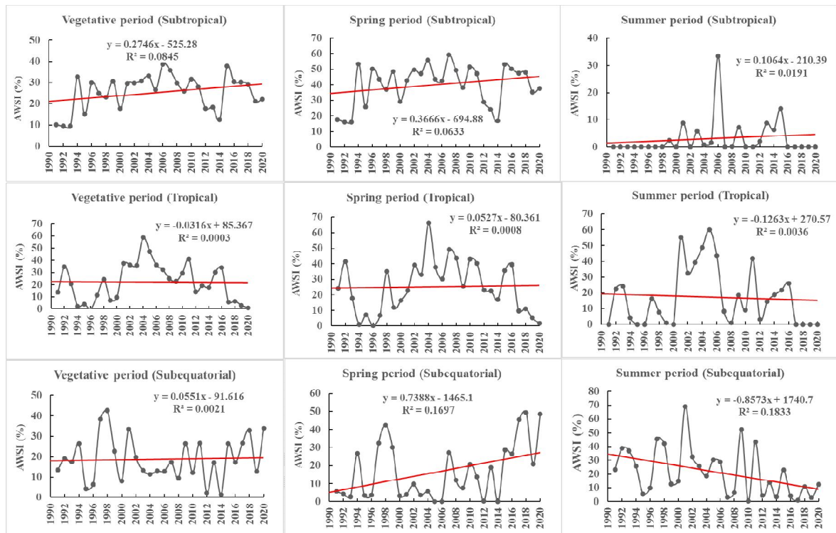
Figure 6: Evolution of the agro-climatic water stress index (AWSI) over the period 1991-2020
