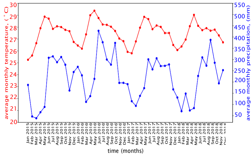
Figure 2: The Philippine climatological data: average monthly temperature (red) and precipitation (blue) for the year 2015–2018.
