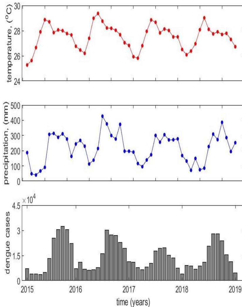
Figure 3: Seasonal variation of the monthly dengue cases and the monthly average temperature and precipitation in the Philippines for the year 2015–2018.
