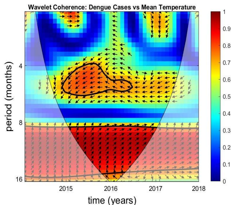
Figure 5: Wavelet coherence analysis between the number of dengue cases and the average temperature (°C).
