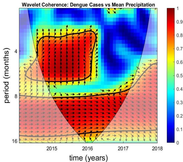
Figure 6: Wavelet coherence analysis between the number of dengue cases and the average precipitation (mm).
