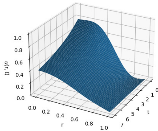
Figure 1: Graph to u(r, t) in Eq. (64) with Q_0 = c = 200, a = 1, \gamma \rightarrow 1 and \kappa = 1 .
