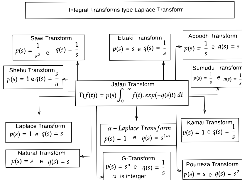
Figure 5: The diagram some particular cases Jafari transform
