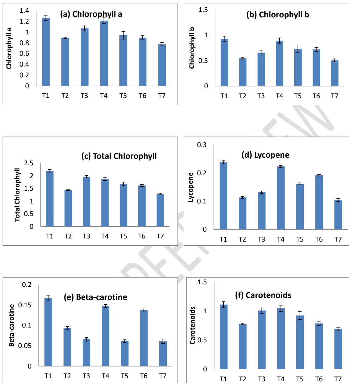
Figure 4. Effects of GA3 priming and exogenous application on the photosynthetic pigments of maize under salt stress. (a) Chlorophyll a; (b) chlorophyll b; (c) total chlorophyll; (d) lycopene; (e) beta-carotene; (f) carotenoids. The error bar represents the standard error.
