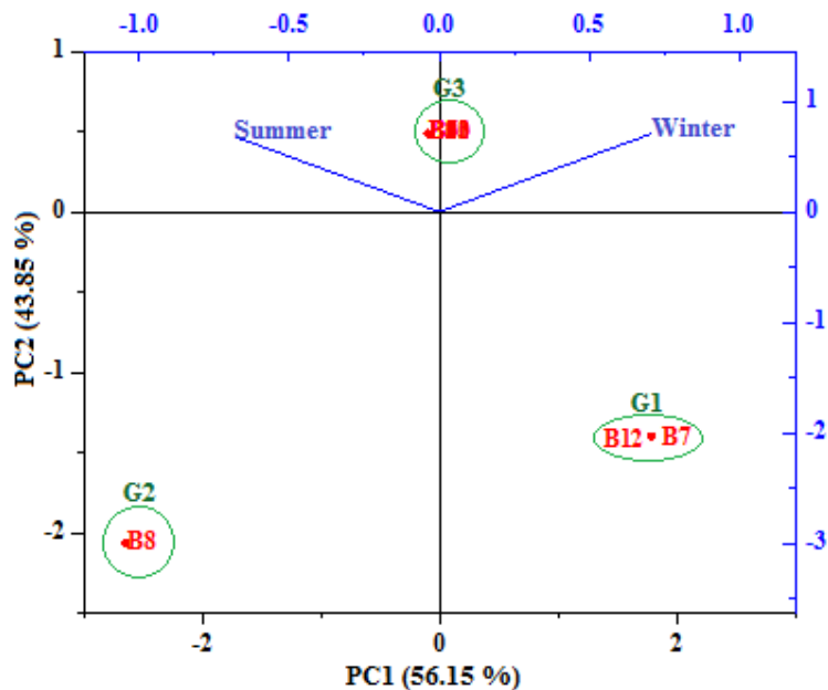
Fig. 4. Biplot diagram between PC1 and PC2 shows similarities and dissimilarities relationships between bands of S. persica during the two seasons. B1-B13: The bands No.1 – No. 13.
