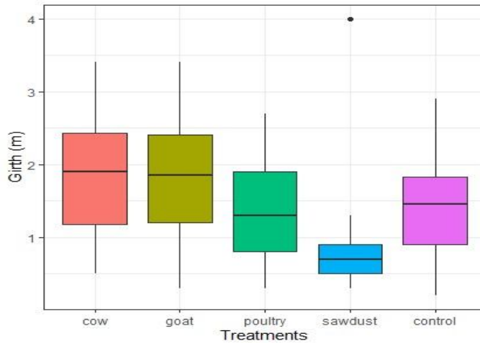
Figure 2. Effect of the different treatments on girth measurement
