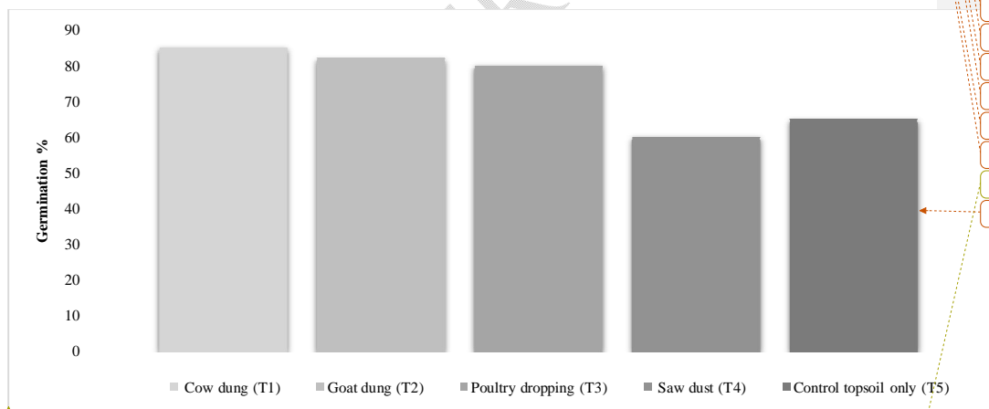
Fig.1: Germination percentage of Newbouldia laevis under different treatments
