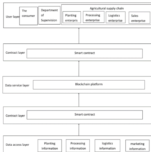
Fig. 2. Smart contract diagram
