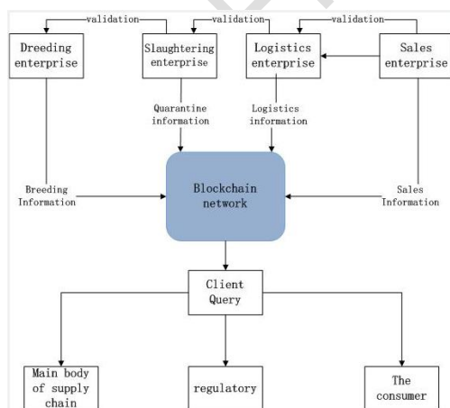
Fig. 4 Blockchain-based traceability model for agricultural products
