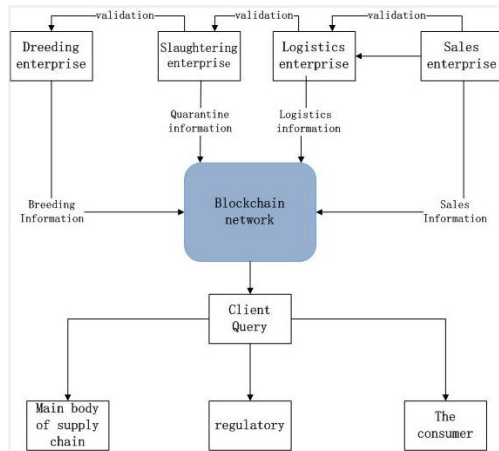
Fig. 3 Blockchain-based traceability model for agricultural products
