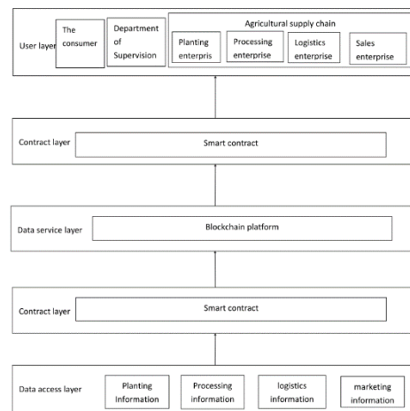
Fig.2. The framework of agricultural product traceability system built by blockchain
