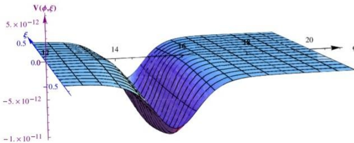
Figure 2. The Ekpyrotic superpotential has been defined in terms of the potentials V(\phi, \xi) which is presented in the paper as V(\phi_0, \phi_1) where V(\phi_1) = 0 for b = \sqrt{3} , d = 1 that in essence shows the decreasing potential \phi_{ekpyrotic} -end with a negative gradient that falls steeply with a saddle-like curvature and bounces back with a non-locally flat curvature satisfying the FLRW [see Appendix B] metric with a small local positive curvature. Source [57].
