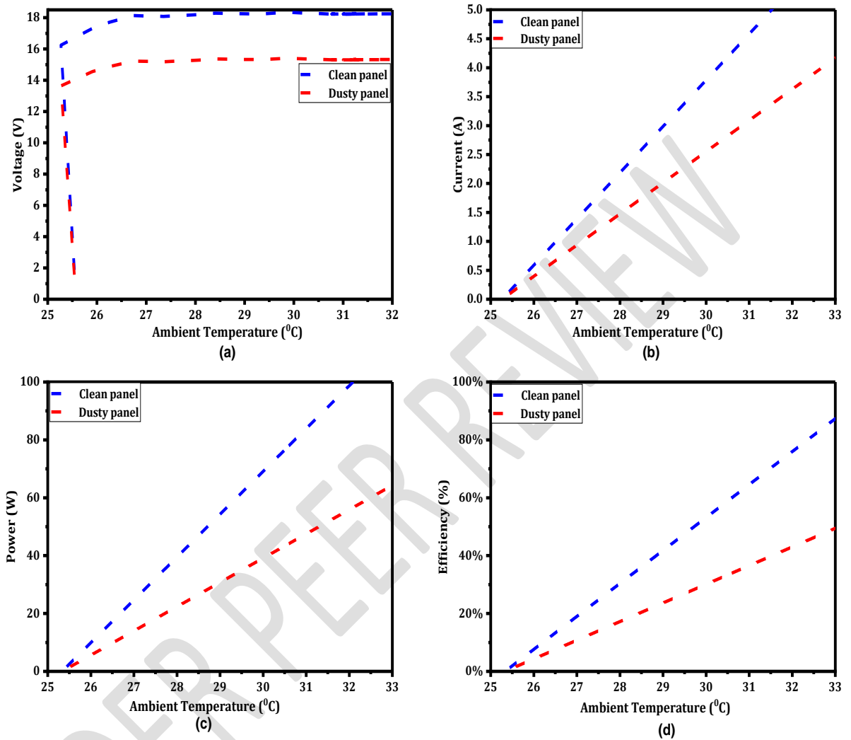
Figure 6: impact of ambient temperature on operating voltage, current, power and efficiency for clean and clean and dusty panels
