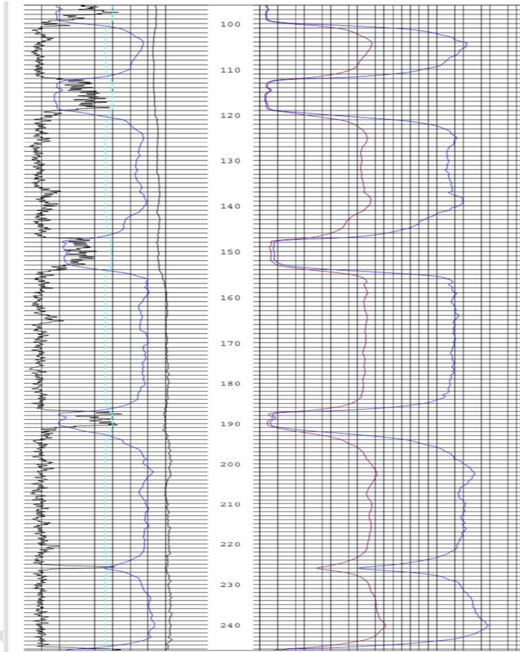
Figure 8: Geophysical Log of a Borehole in IMT/OSB
