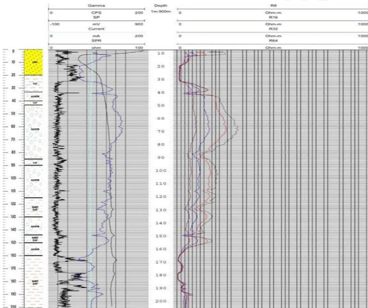
Figure 5 : Geophysical Log of a Borehole at Ngo, Andoni LGA
