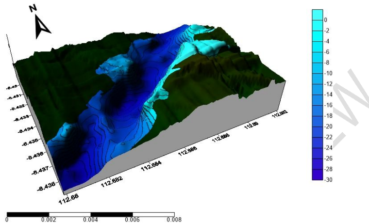
Fig.2. Bathymetry at tourism zone Sendang Biru waters and Sempu Island
