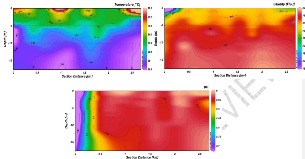
Fig.6. Transverse profile of temperature, salinity, and pH
