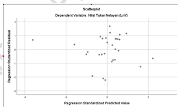
Fig. 2. Heteroscedasticity assumption test results
