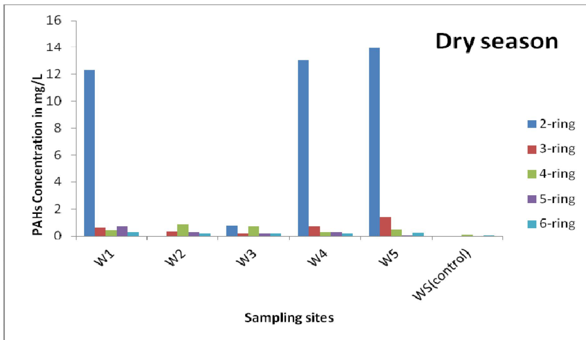
Fig. 2.: Analysis of the PAH concentration results based on number of rings for underground water around Edem Udo (W1), Etebi Idung Iwak (W2), Nkubia (W3), Grace Bill (W4) and RCC (W5) automobile repair workshop and Control sample (WS) during dry season
