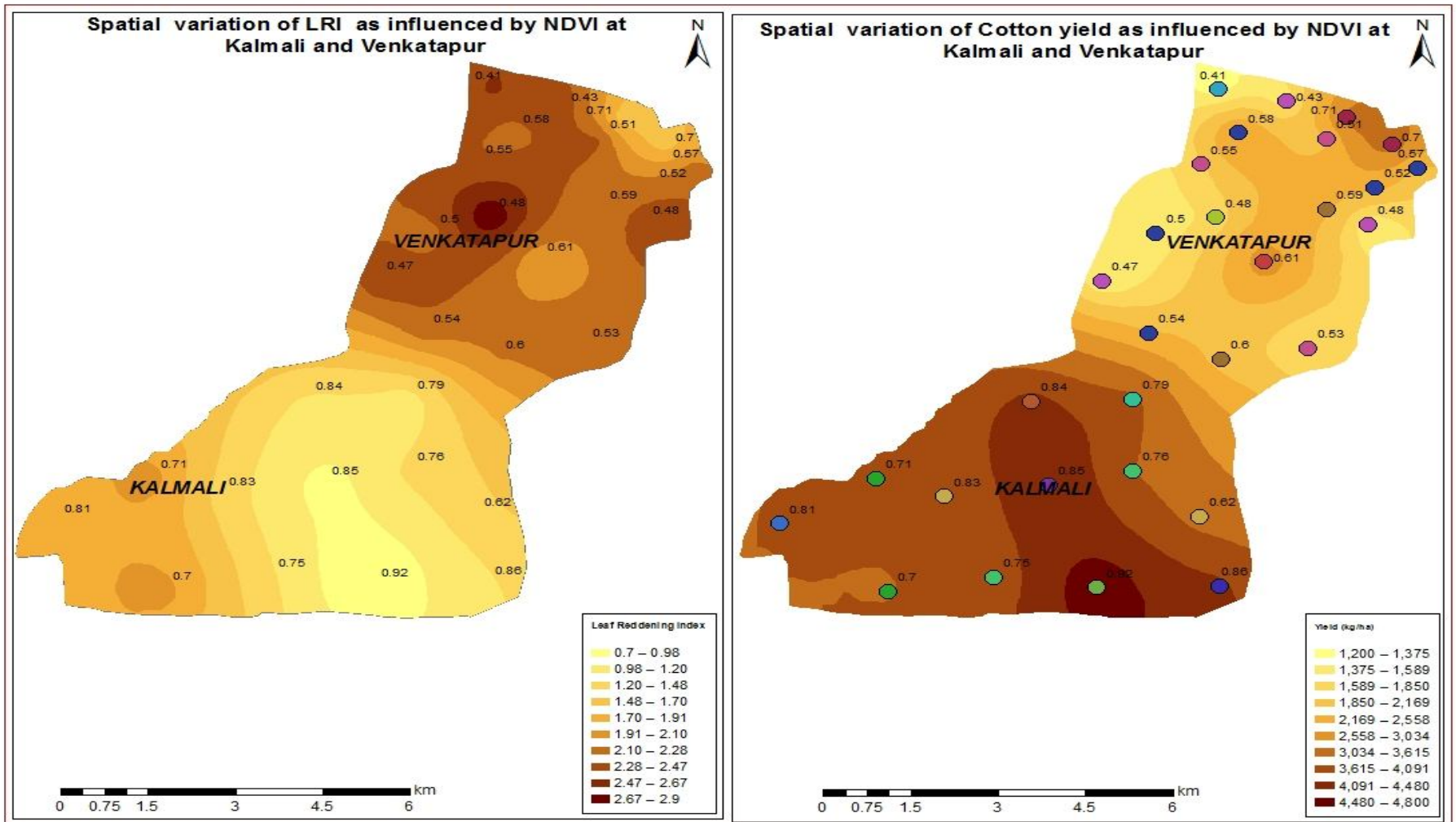
Fig. 5: Spatial variation of leaf reddening index and cotton yield with respect to NDVI values at Kalmali and Venkatapur village
