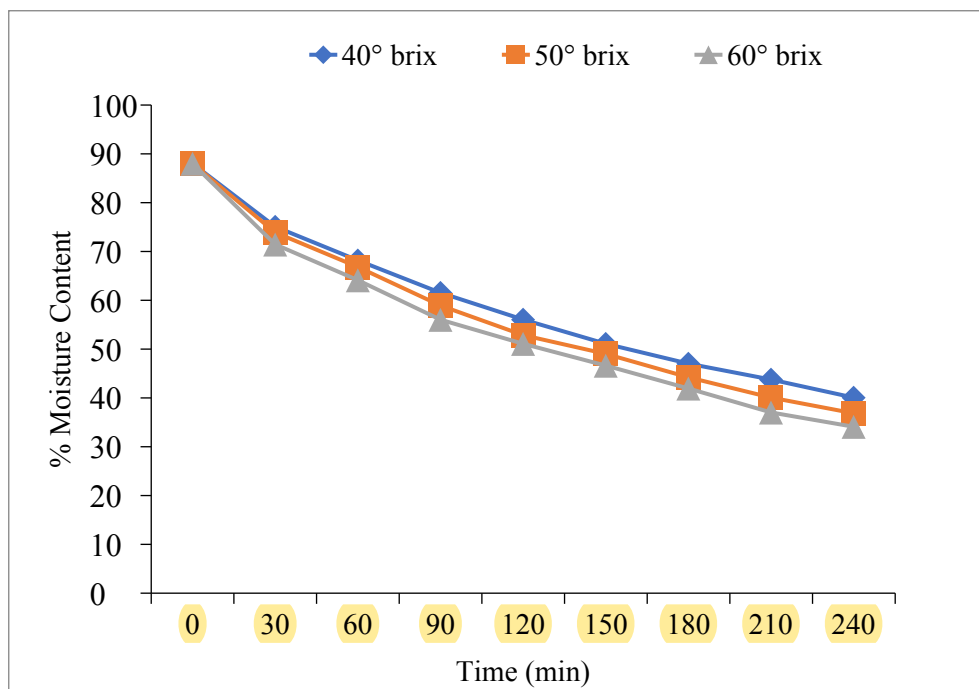
Figure 2 a. Moisture reduction behavior of 0.5 cm thick
