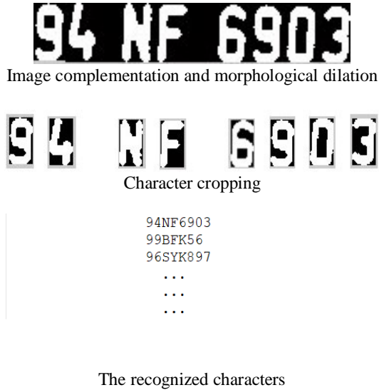
Fig. 10. The produced images in LPR stage
