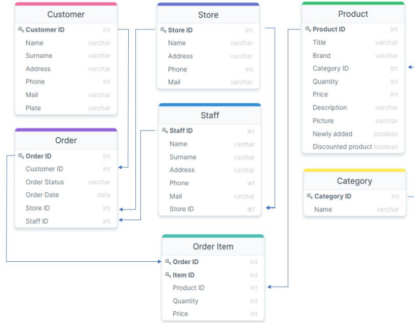
Fig. 11. Proposed DB's tables
