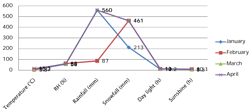
Fig.-10: Weather Report of Poonch District of Jammu & Kashmir for the Month of January to April-2022
