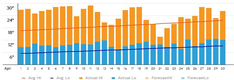
Fig.-09: Temperature graph of Poonch District of Jammu & Kashmir for the Month of April-2022
