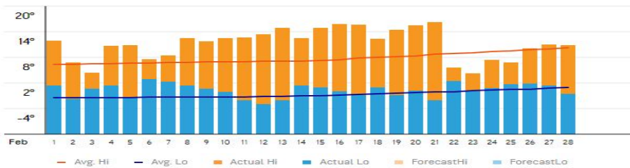
Fig.-07: Temperature graph of Poonch District of Jammu & Kashmir for the Month of February-2022
