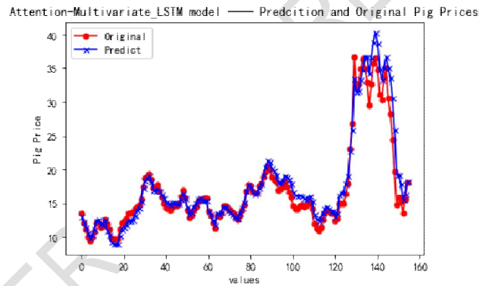
Fig. 7 Attention- Multivariable_LSTM model
