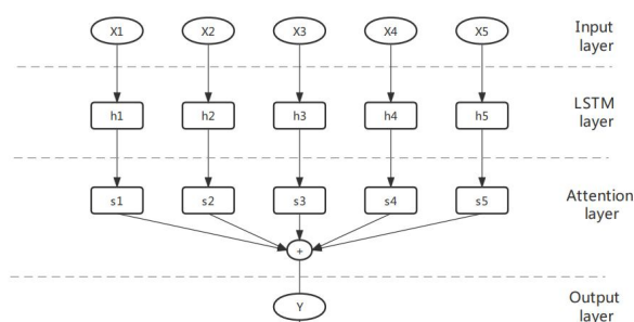
Fig. 5 Attention-LSTM structure diagram
