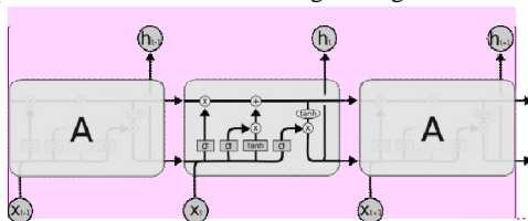
Fig. 3 LSTM structure diagram
