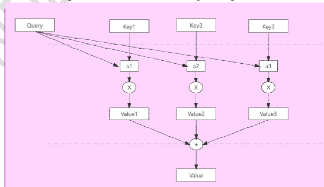
Fig. 4 essential idea of Attention mechanism
