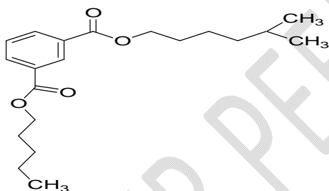
Isophthalic acid 1-(5-methyl-hexyl) ester 3-pentyl ester
