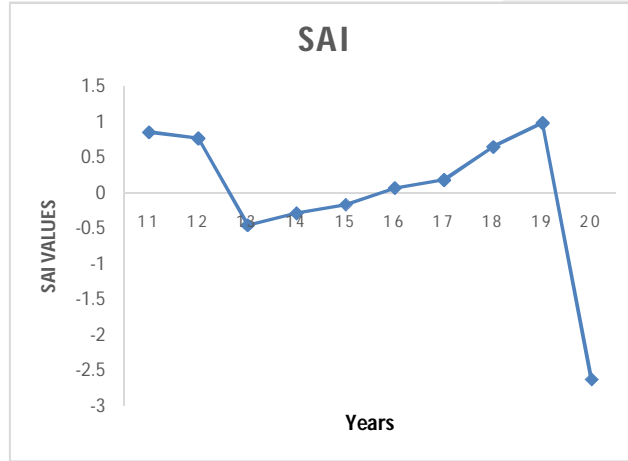
Fig 5: Decadal rainfall from 2010 to 2020
