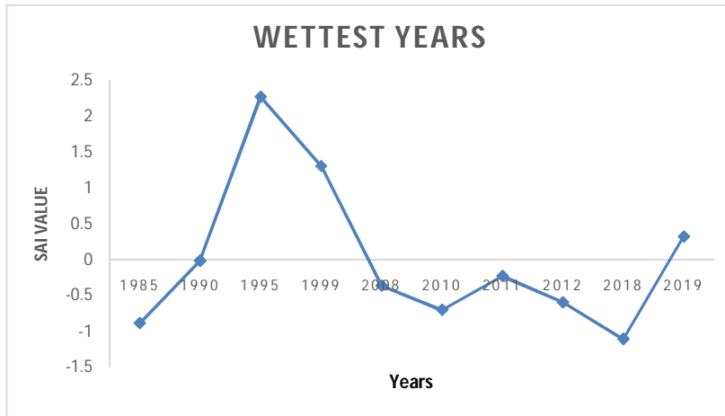
Fig 6b: wettest rainfall analysis
