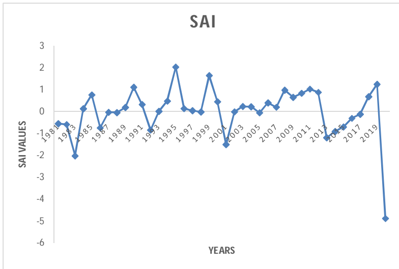
Fig 6a: wettest rainfall analysis
