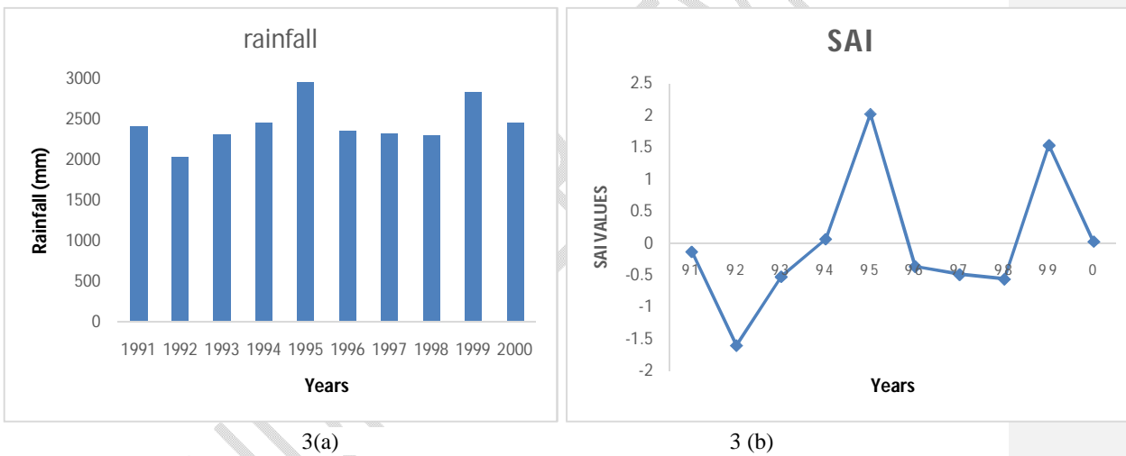
Fig 3: Decadal rainfall from 1991 to 2000
