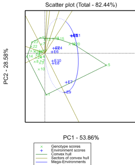
1 2 Figure 1: Polygon view of the GGE-biplot for the which – one – where pattern for genotypes and 3 environments
