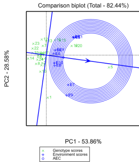
Figure 4: GGE-biplot with scaling focused on environments
