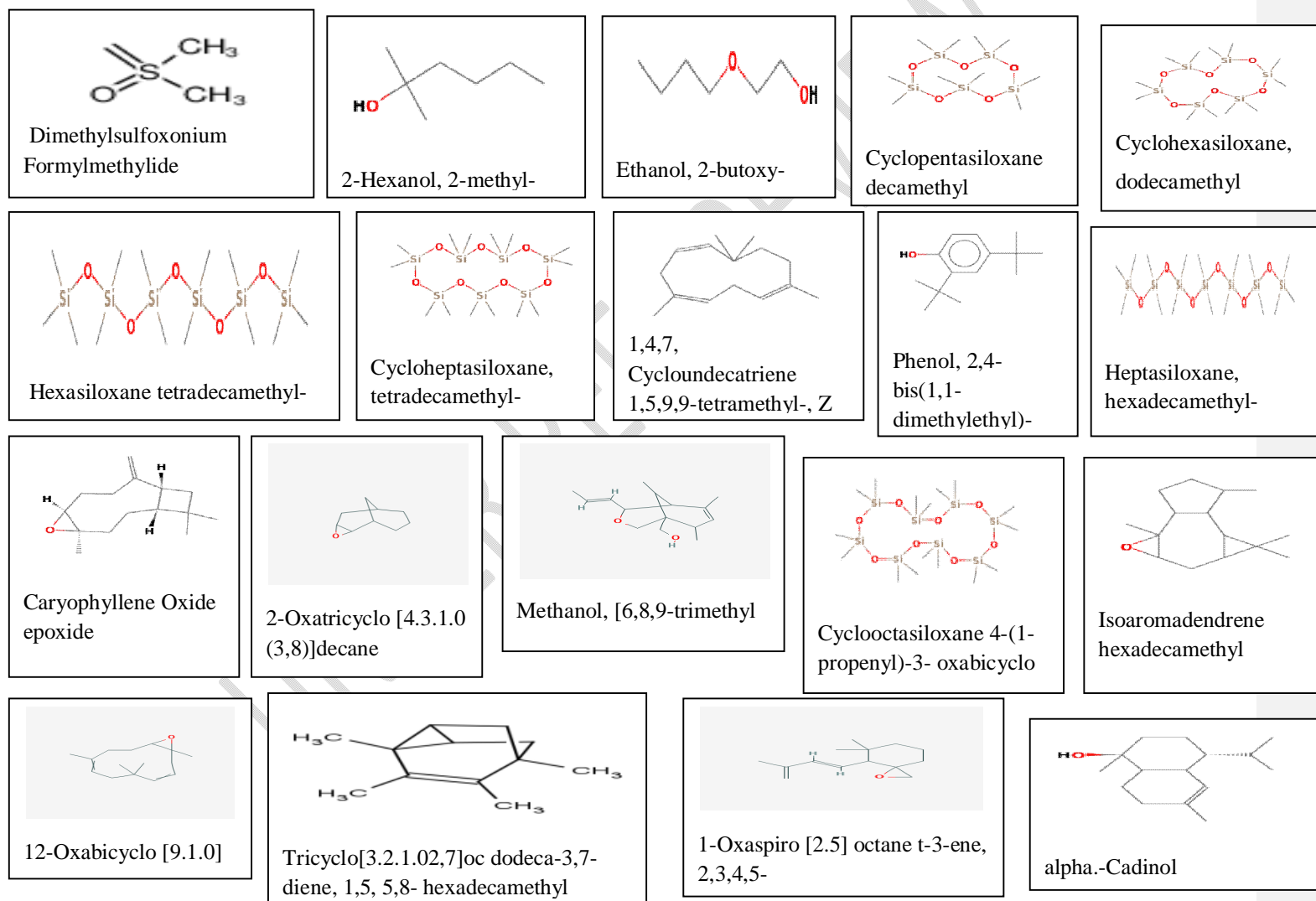
Figure 14: Summary of Gas chromatography and mass spectroscopy (GC-MS) Analysis of Aframomum melegueta stem extract of Purified Essential oil stem extract (SD++)
