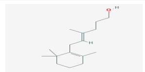
4-Hexen-1-ol, 6-(2,6,6-trimethyl-1-cyclohexen)
