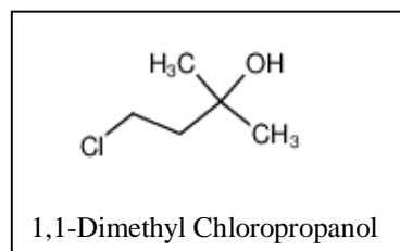
figure 12 : Summary of Gas chromatography and mass spectroscopy (GC-MS) Analysis of Aframomum melegueta stem
