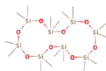
Cyclooctasiloxane, hexadecamethyl-
