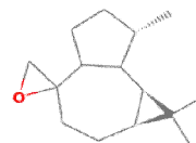
Alloaromadendrene oxide-(1)
