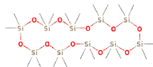
Cyclodecasiloxane eicosamethyl-
