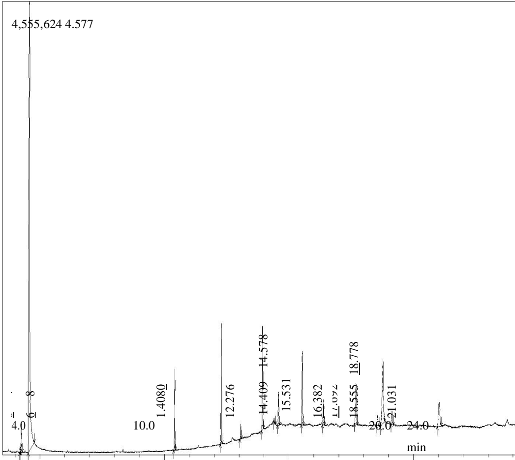
Figure 11 : Spectral 1;Gas chromatography and mass spectroscopy(GC-MS) Spectra Analysis of Aframomum melegueta Purified Essential oil stem extract (Std+)
