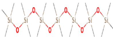
Heptasiloxane, hexadecamethyl-
