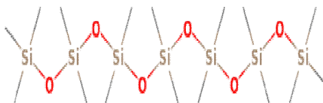
Heptasiloxane, hexadecamethyl-
