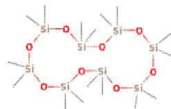
Cyclooctasiloxane, hexadecamethyl-
