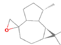
Alloaromadendrene oxide-(1)
