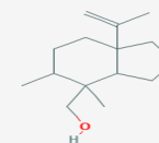
(7a-Isopropenyl-4,5-dimethyloctahydroinden
