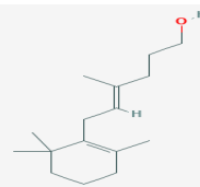
4-Hexen-1-ol, 6-(2,6,6-trimethyl-1-cyclohexen
