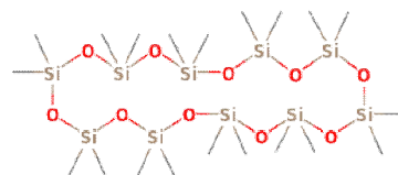
Cyclodecasiloxane eicosamethyl-
