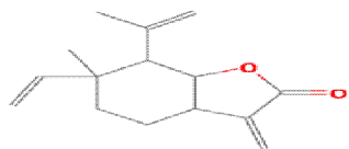
2(3H)-Benzofuranone 6-ethenylhexahydro-6-
