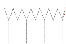
2-Pentadecanone 6.10.14-trimethyl
