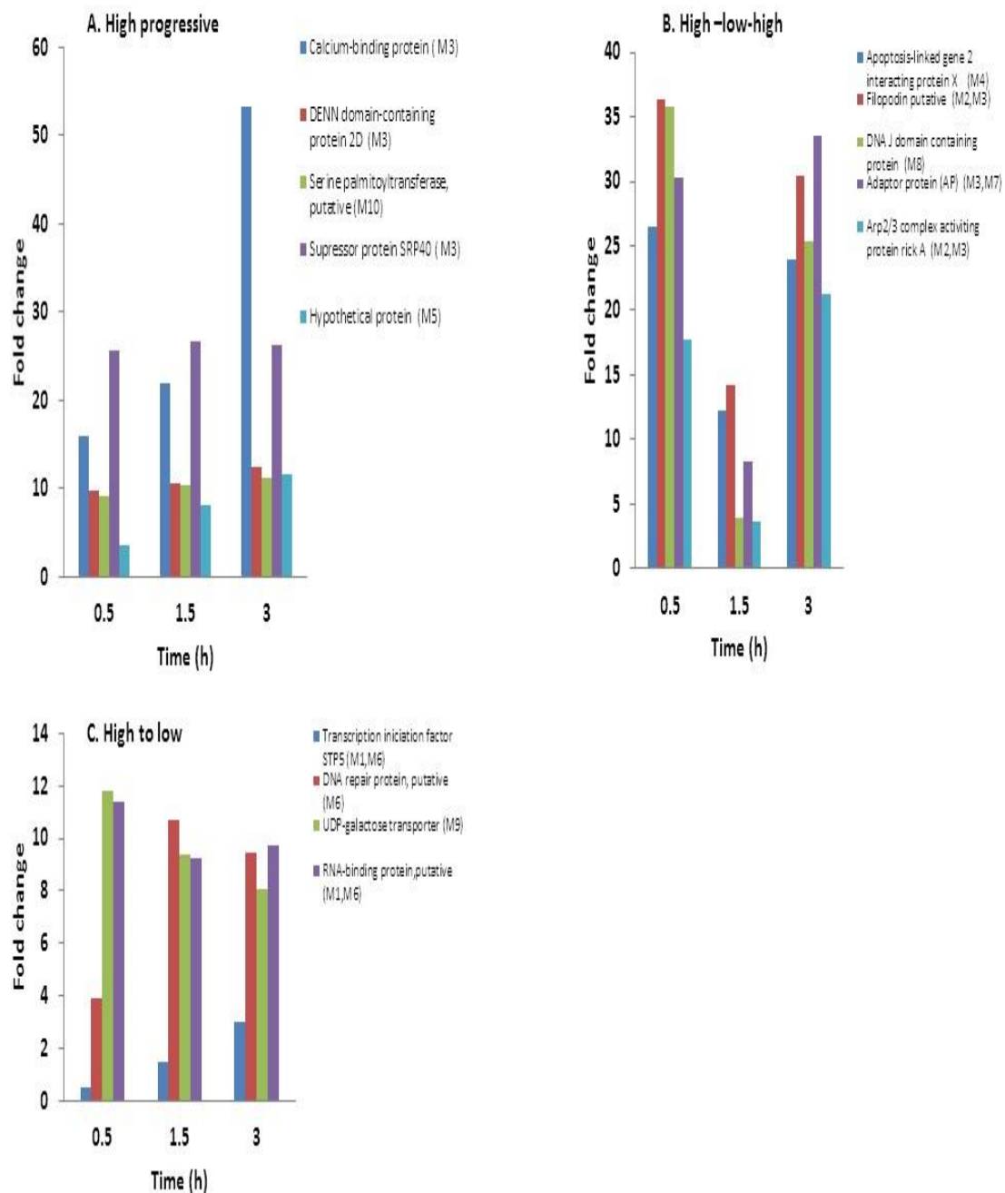
Figure 3. Expression pattern profiles of representative up-regulated genes from some modules.
