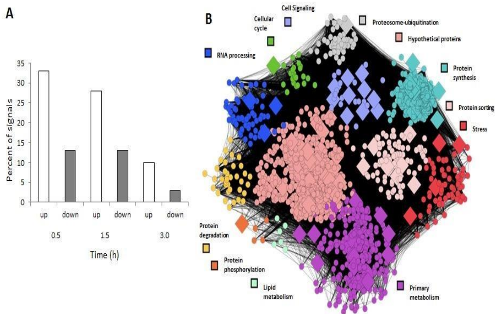
Figure 1. Signals modulated during host-parasite interactions A. Expression percentage of genes at each time of host-parasite interaction. Each bar indicates the percentage of genes that are upregulated or downregulated from microarray analysis. B. Graphic representation of the network analysis.
