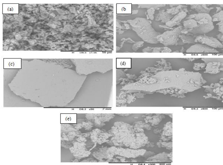
Figure 5. SEM images of (a) GLB, (b) HPMC, (c) PEG-8000, (d) Na-citrate and (e) GCHP-4.
