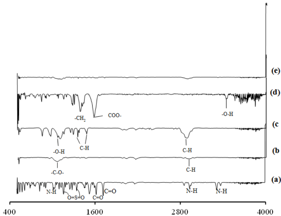
Figure 4 FT-IR spectra of (a) GLB, (b) HPMC, (c) PEG-8000, (d) Na-citrate and (e) GCHP-4
