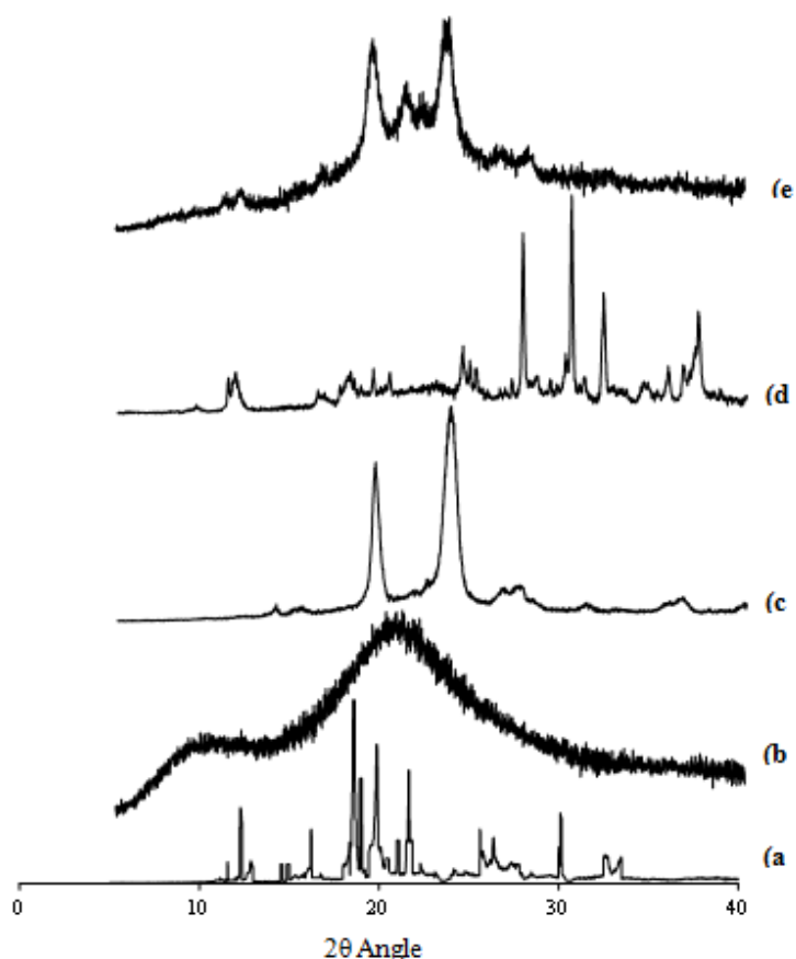
Figure 3. Powder X-ray diffraction patterns of (a) GLB, (b) HPMC, (c) PEG-8000, (d) Na-citrate; and (e) GCHP-4.
