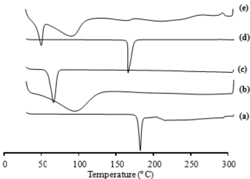
Figure 2. DSC thermograms of (a) GLB, (b) HPMC, (c) PEG-8000, (d) Na-citrate and (e) GCHP-4.
