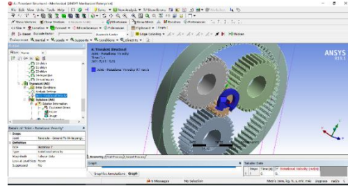
Fig. 9. Add torque to the center gear.
