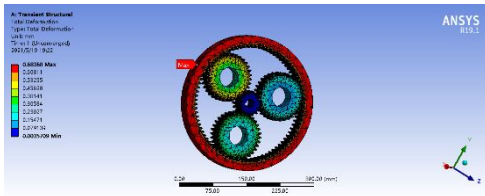
Fig. 11. The model deformation cloud image.
