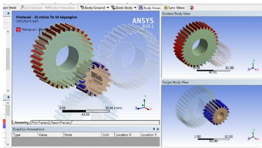
(a) Contact between planetary gear and center gear.
